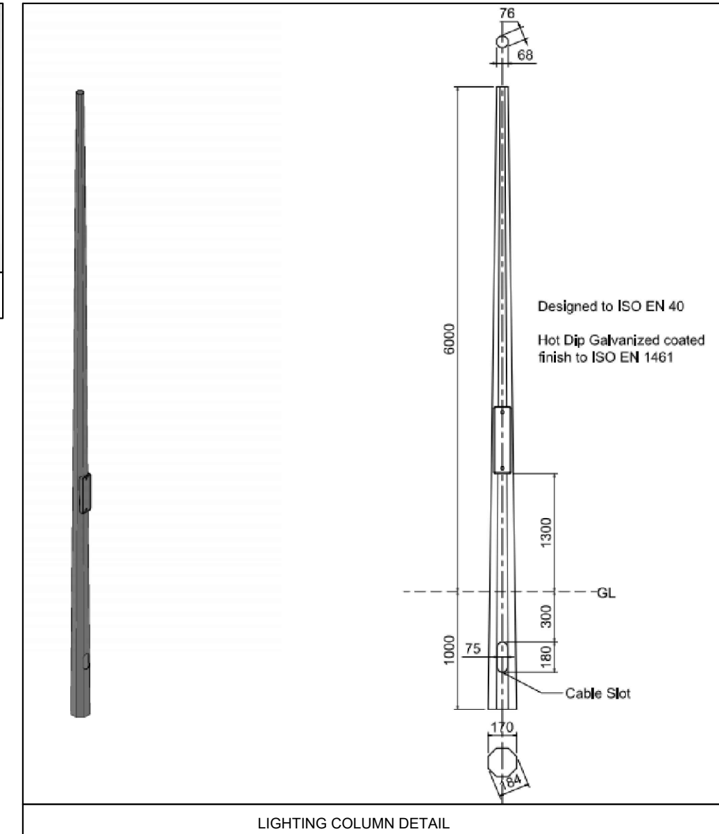
LIGHTING COLUMN DETAIL
