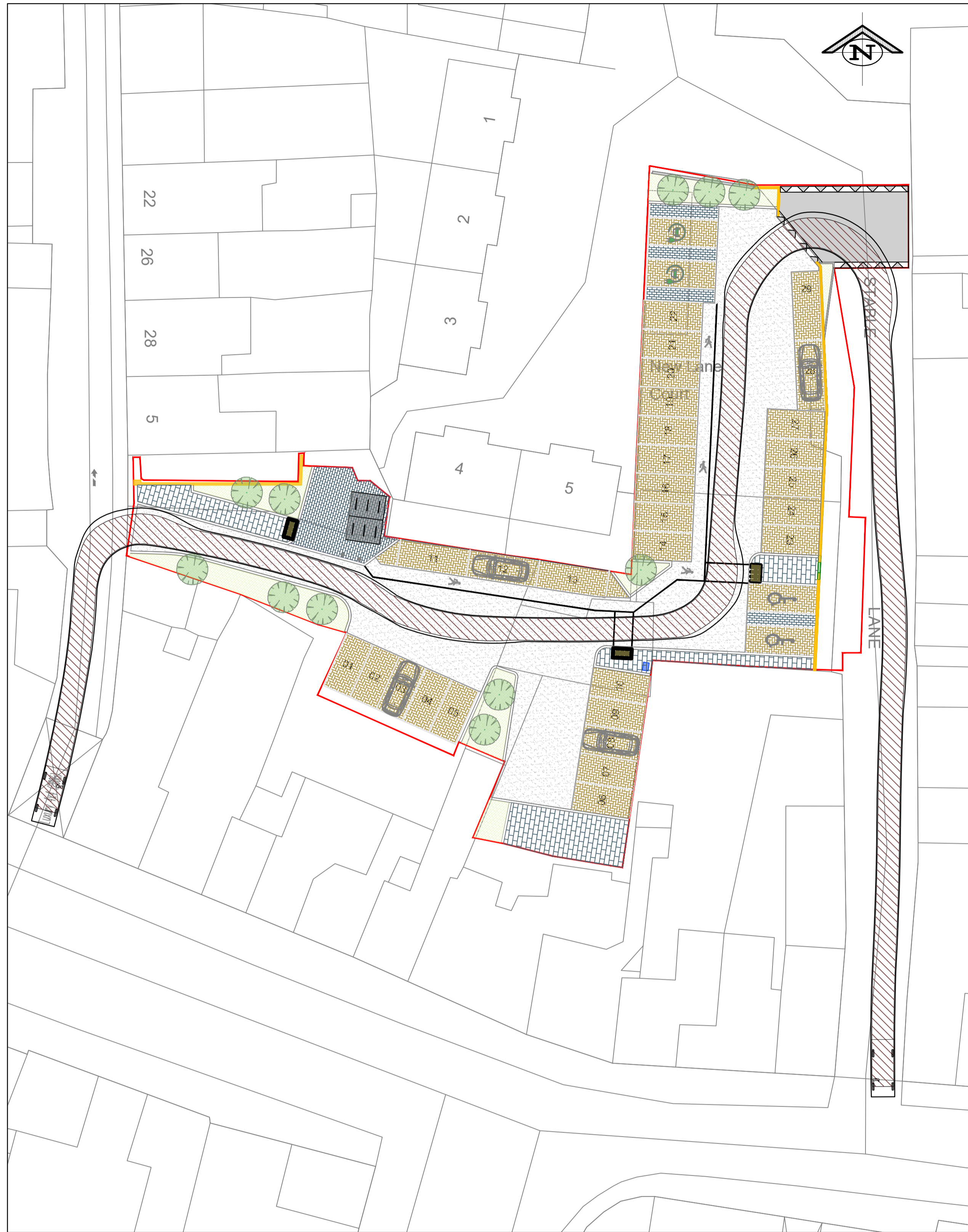
STABLE LANE CARPARK - AUTO-TRACKING IN & OUT OF CARPARK SCALE 1:250
