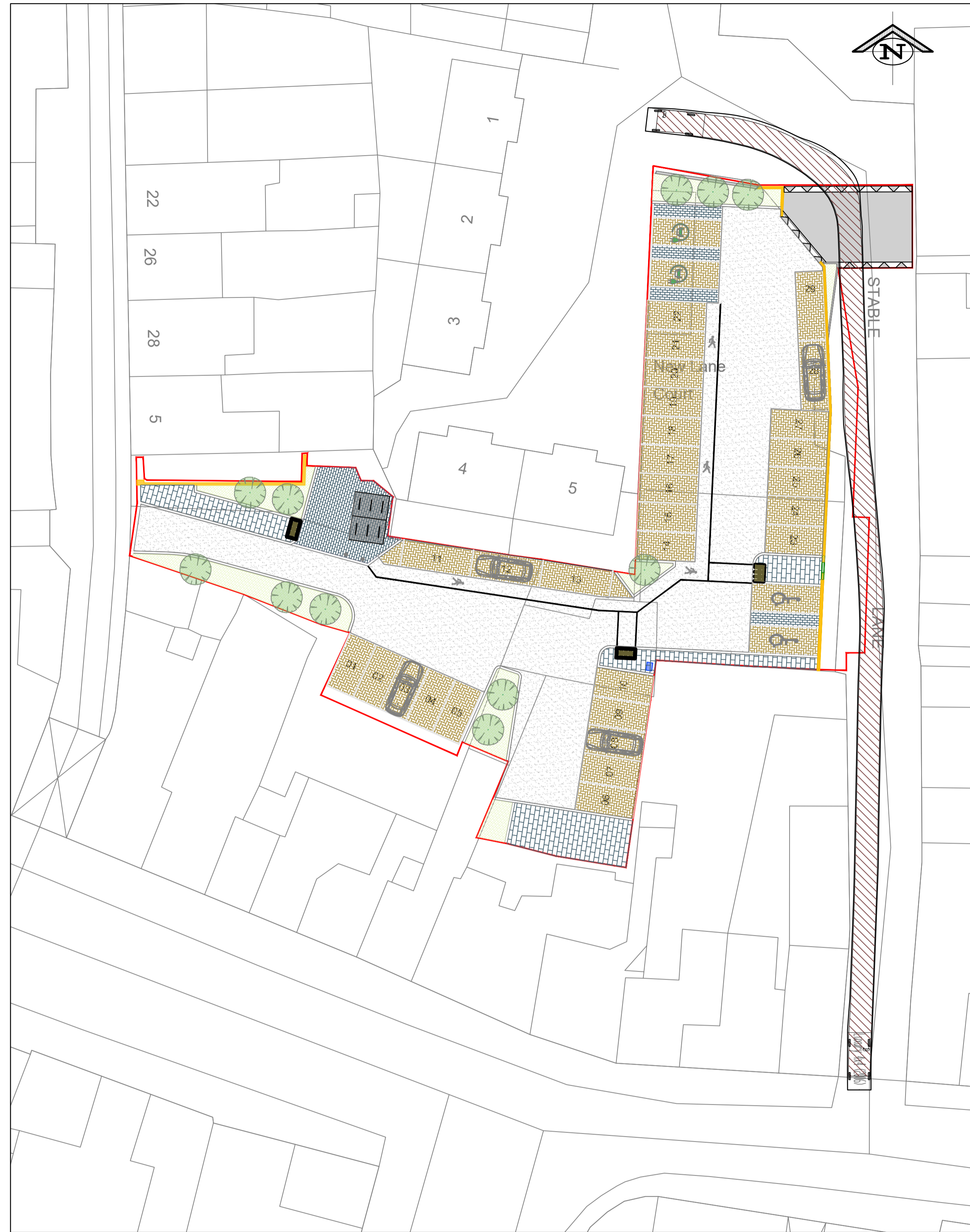
STABLE LANE CARPARK - AUTO-TRACKING INTO HOUSING AT REAR SCALE 1:250
