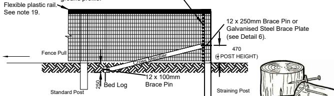
DETAIL 2 - END POST ASSEMBLY ELEVATION
