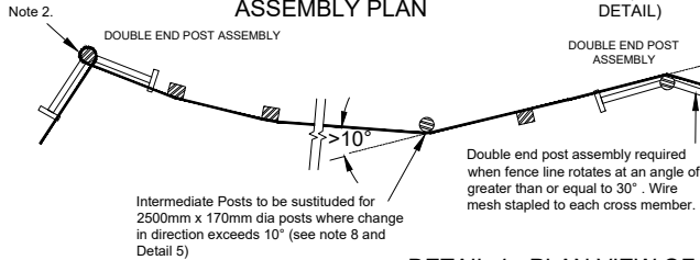
DETAIL 4 - PLAN VIEW OF CURVED FENCELINE STRAINING POST & END POST ASSEMBLY REQUIREMENTS
