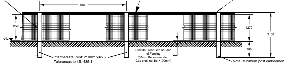
FENCE ELEVATION FENCE PLAN
