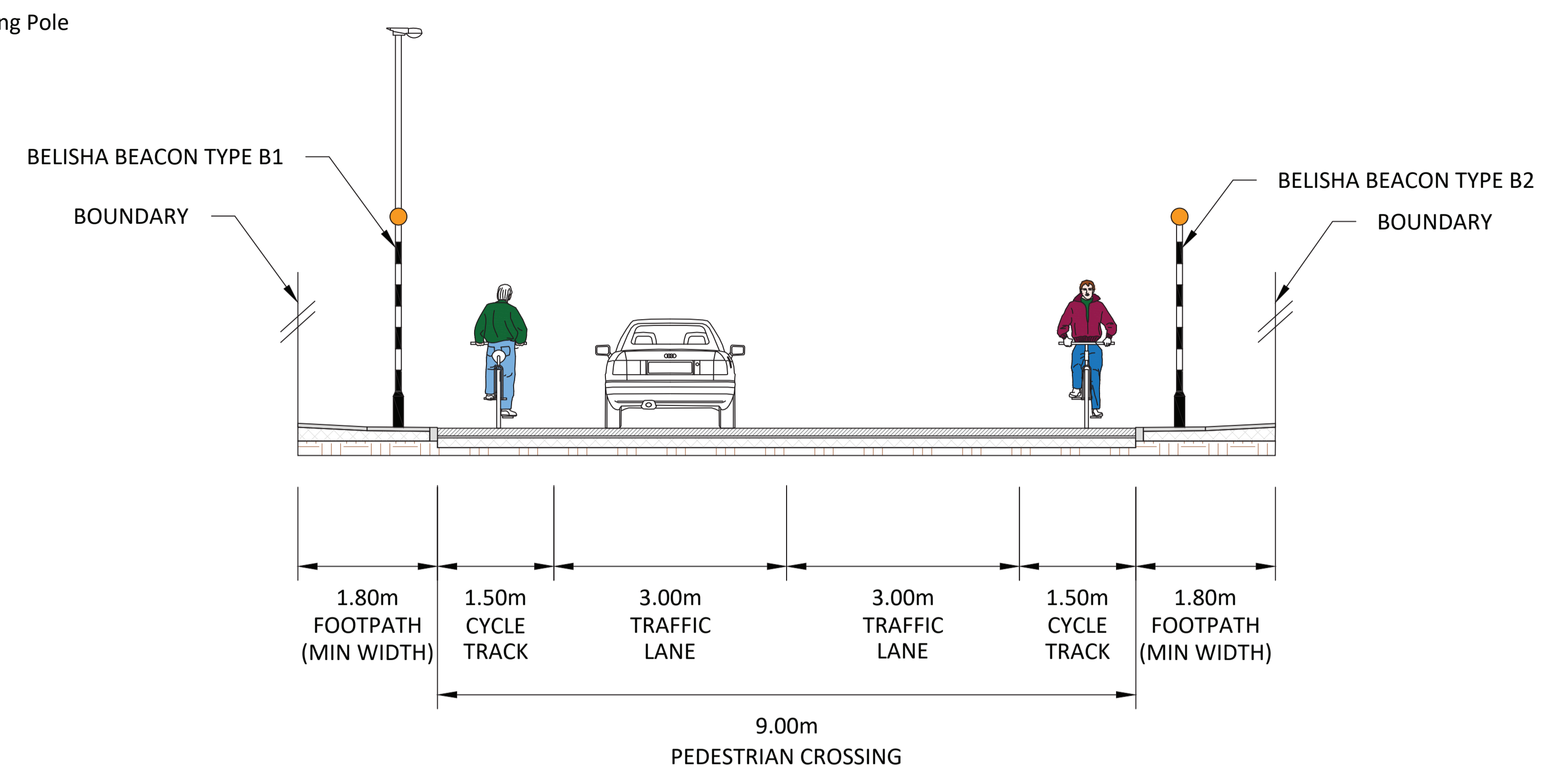
TYPICAL CROSS SECTION C-C 1:50
