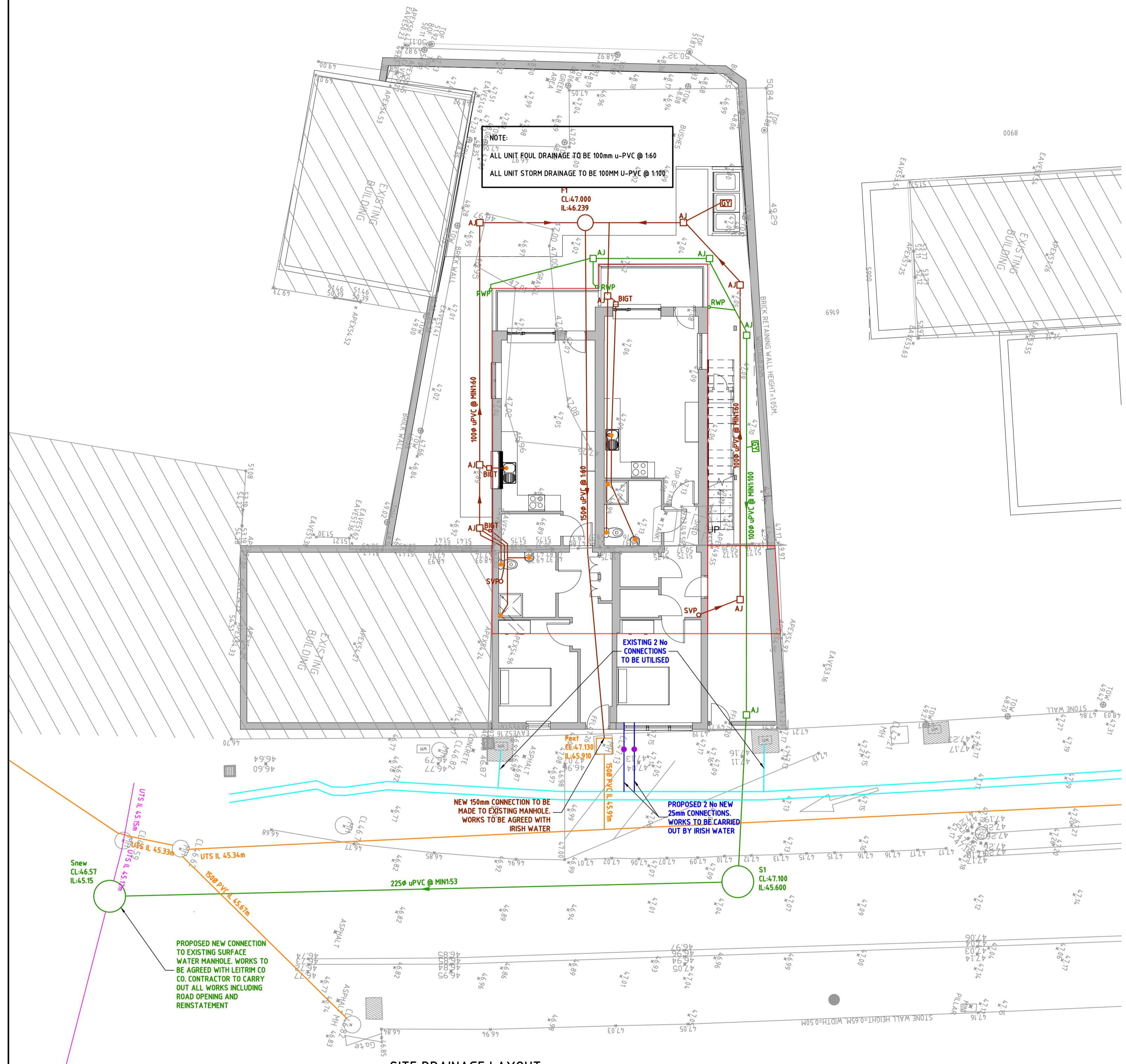
SITE DRAINAGE LAYOUT SCALE 1:100
