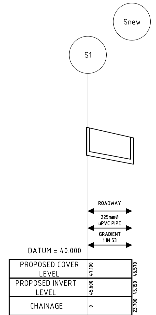
PROPOSED STORM SEWER SECTIONS S1-Snew HORIZONTAL SCALE 1:100 VERTICAL SCALE 1:100
