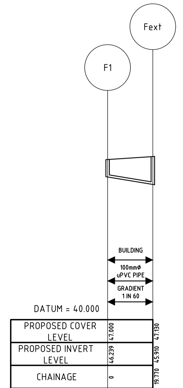
PROPOSED FOUL SEWER SECTIONS F1-Fext HORIZONTAL SCALE 1:100 VERTICAL SCALE 1:100
