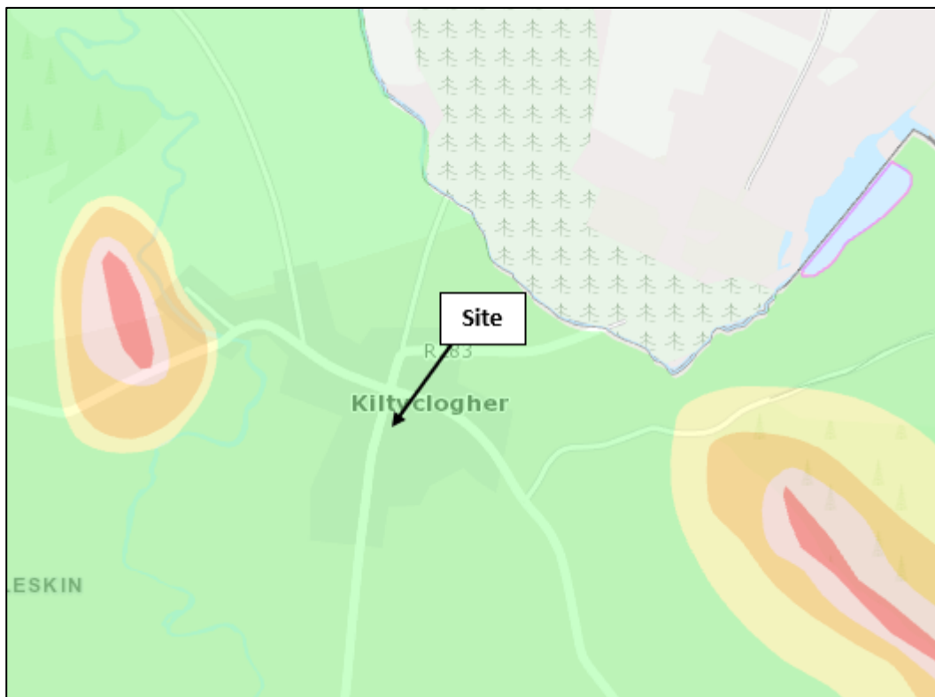
Figure 4.2: Groundwater Vulnerability
