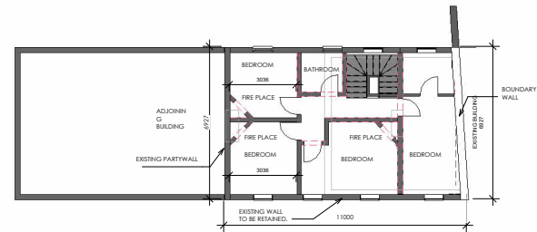
6 FIRST FLOOR 1 : 100
