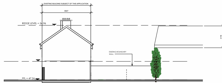
1 SIDE NORTH 1 : 100
