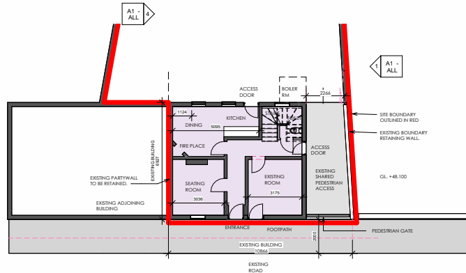
5 GROUND FLOOR 1 : 100
