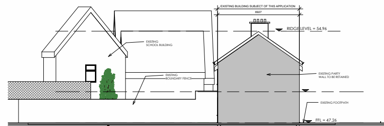
4 SIDE SOUTH 1 : 100
